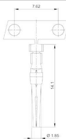
Crimp Socket connector
