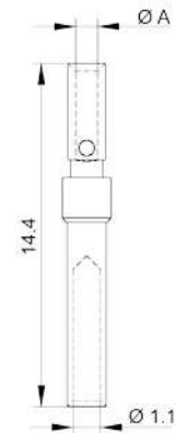
Crimp Socket connector
