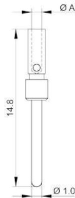
Crimp Plug connector
